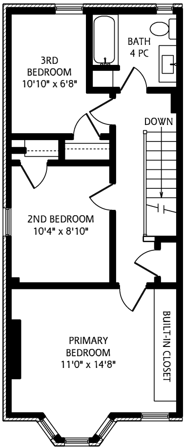
SECOND FLOOR 600 SQUARE FEET
