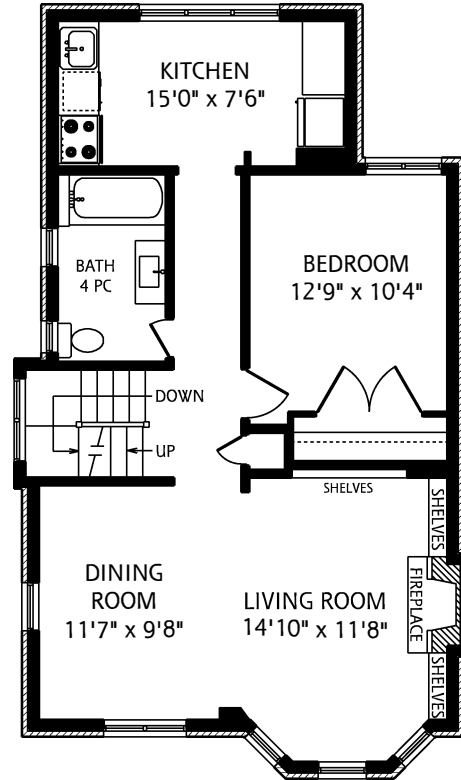
SECOND FLOOR 840 SQUARE FEET
