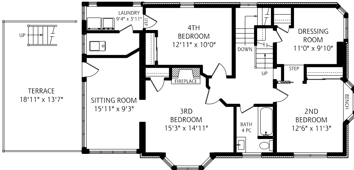
SECOND FLOOR 1,265 SQUARE FEET
