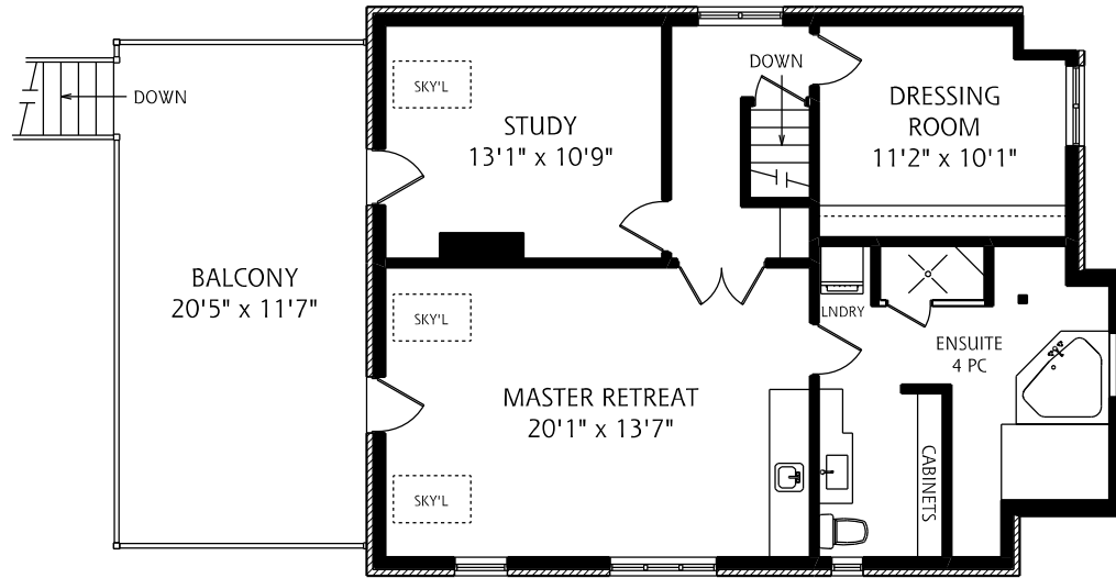
THIRD FLOOR 925 SQUARE FEET
