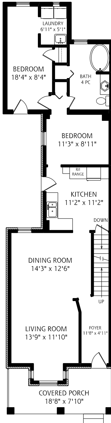
MAIN FLOOR 1,110 SQUARE FEET
