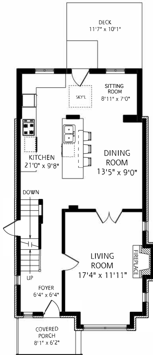
MAIN FLOOR 810 SQUARE FEET
