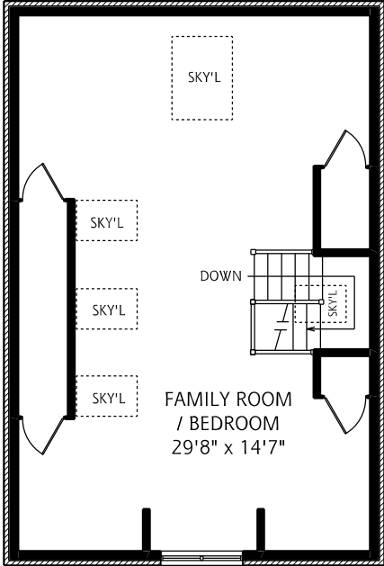
THIRD FLOOR 800 SQUARE FEET
